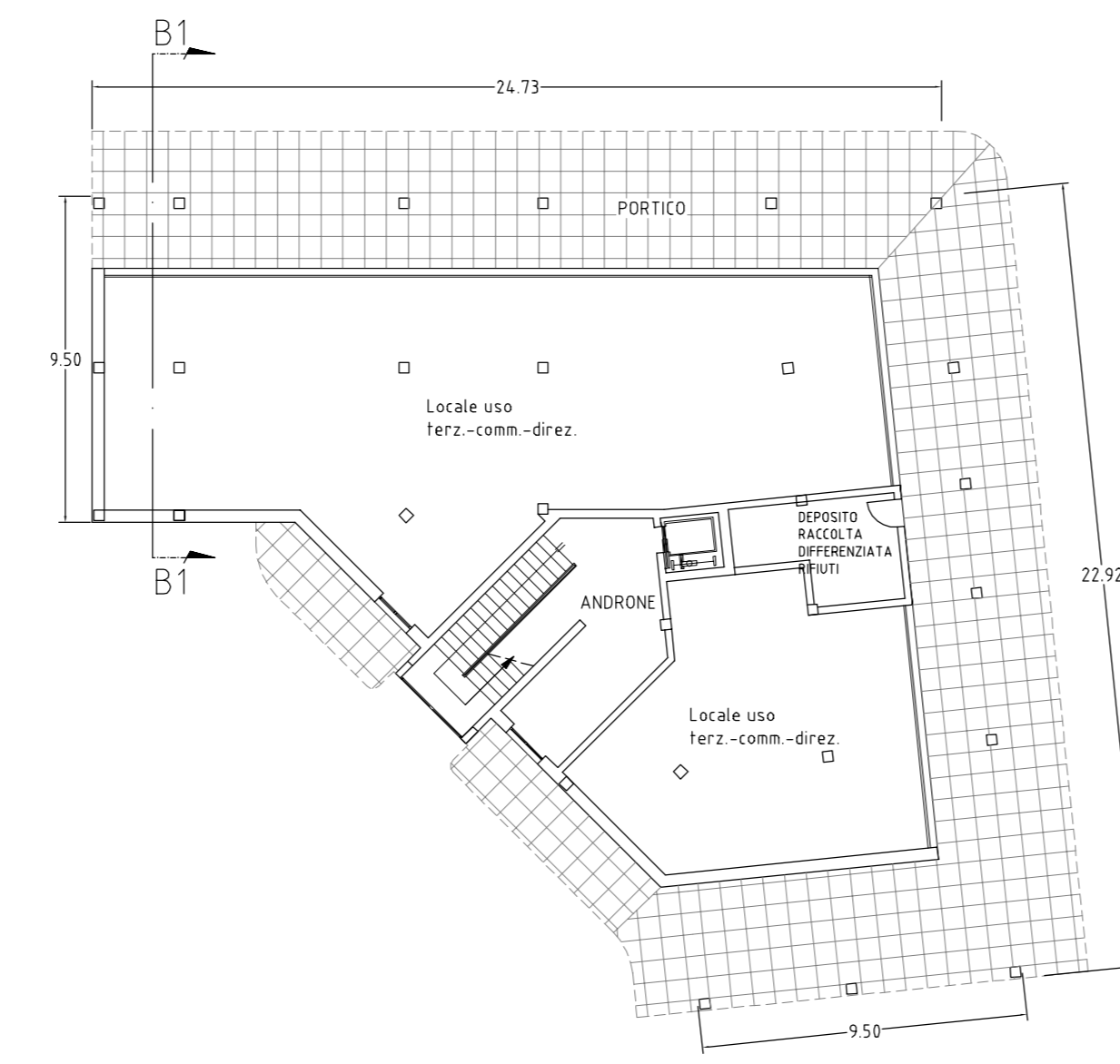
PIANTA PIANO I
