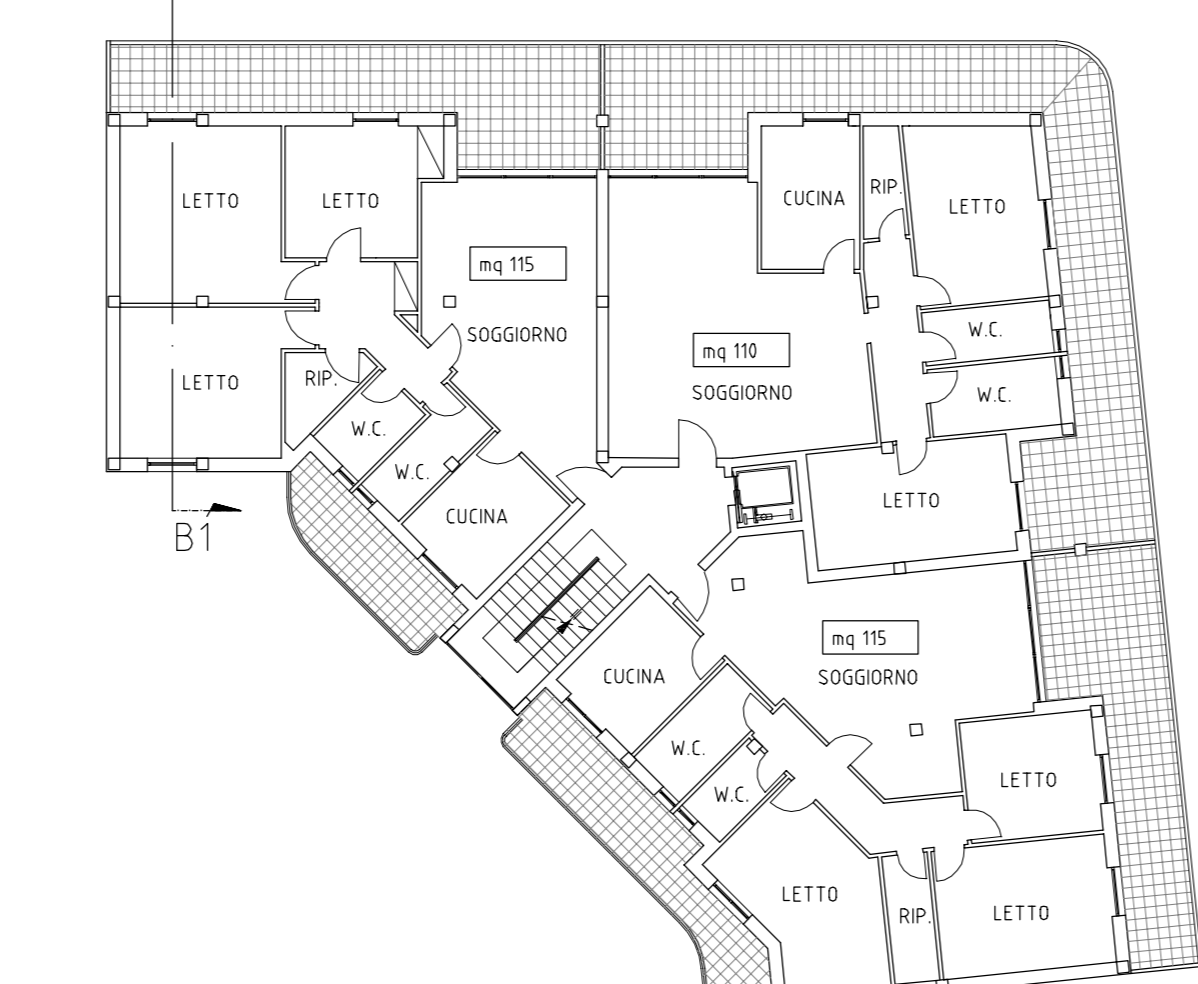
PIANTA PIANO I
