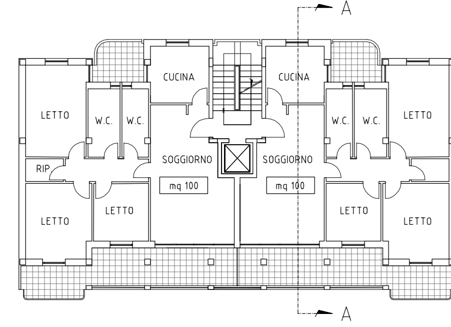
PIANTA PIANO V
