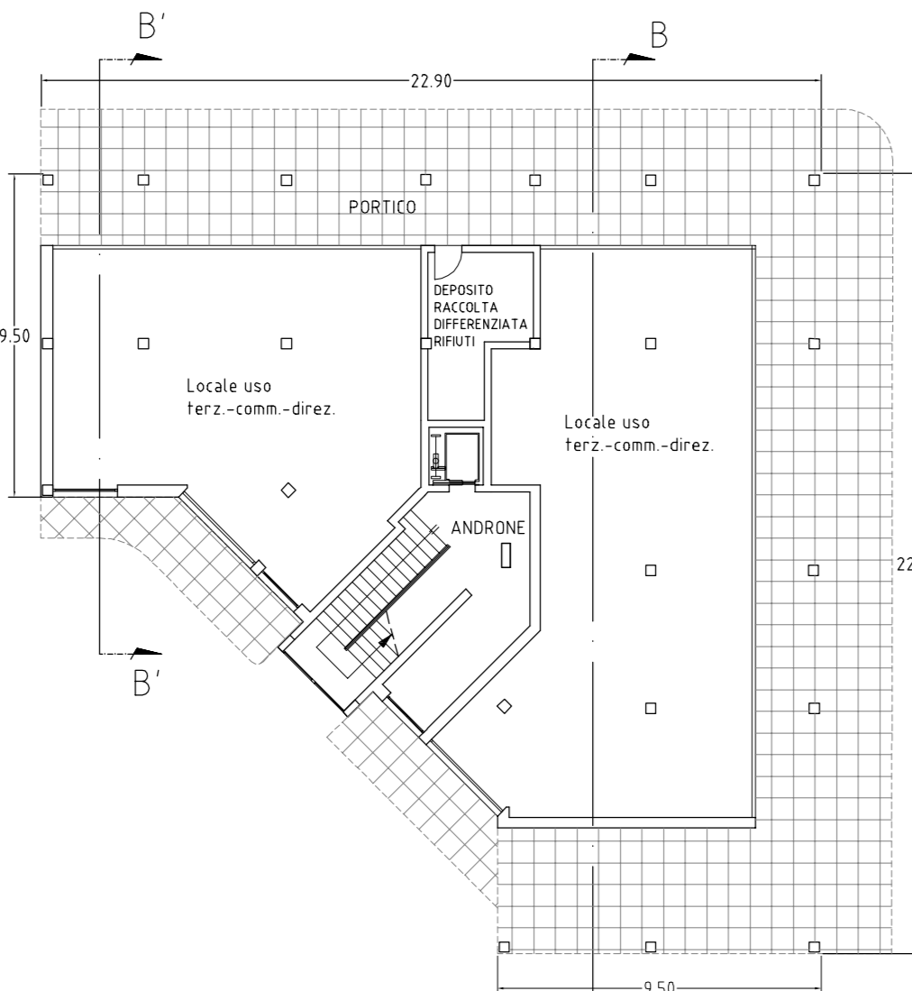
PIANTA PIANO I
